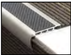
AA121 1 1/2" Bullnose BULLNOSE SAFETY STAIR WITH PRE-DRILLED AND COUNTER-SUNK HOLES FOR #4 SCREW 82° INSERT WIDTH: 43MM FINISH: EA, EN, BRZ
