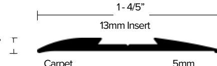
DT029 Carpet to LVT Transition SAFETY TRANSITION FOR USE BETWEEN 5MM LVT AND CARPET. PRE-DRILLED AND COUNTER-SUNK HOLES FOR #4 SCREW 82° INSERT WIDTH: 13MM FINISH: EA, EN, BRZ, EBLK
