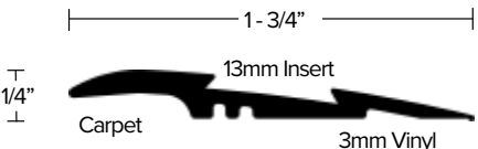
DT027 Carpet to LVT Transition SAFETY TRANSITION FOR USE BETWEEN 3MM LVT AND CARPET. PRE-DRILLED AND COUNTER-SUNK HOLES FOR #4 SCREW 82° INSERT WIDTH: 13MM FINISH: EA, EN, BRZ, EBLK
