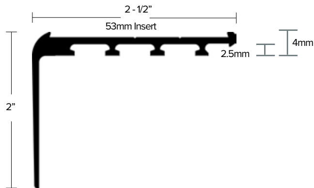
AA123 2" Right Angle Drop SAFETY STAIR WITH PRE-DRILLED AND COUNTER-SUNK HOLES FOR #4 SCREW 82° INSERT WIDTH: 53MM FINISH: EA, EN, BRZ, EBLK
