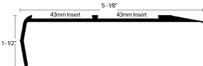
AA207 Extended Bare Floor Nosing SAFETY STAIR WITH PRE-DRILLED AND COUNTER-SUNK HOLES FOR #4 SCREW 82° INSERT WIDTH: 43MM X 2 FINISH: EA, EN, BRZ, EBLK
