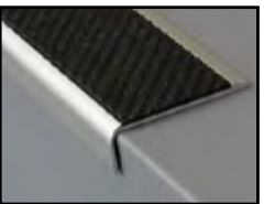
AA125 1" Rake-Back SAFETY STAIR WITH PRE-DRILLED AND COUNTER-SUNK HOLES FOR #4 SCREW 82° INSERT WIDTH: 53MM FINISH: EA, EN, BRZ
