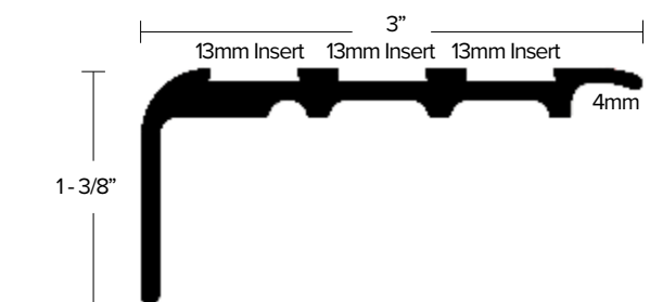
AA346 1 3/8" Right Angle Drop SAFETY STAIR WITH PRE-DRILLED AND COUNTER-SUNK HOLES FOR #4 SCREW 82° INSERT WIDTH: 13MM X 3 FINISH: EA, EN, BRZ
