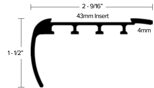
AA121 1 1/2" Bullnose BULLNOSE SAFETY STAIR WITH PRE-DRILLED AND COUNTER-SUNK HOLES FOR #4 SCREW 82° INSERT WIDTH: 43MM FINISH: EA, EN, BRZ
