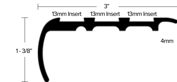
AA345 1 3/8" Bullnose BULLNOSE SAFETY STAIR WITH PRE-DRILLED AND COUNTER-SUNK HOLES FOR #4 SCREW 82° INSERT WIDTH: 13MM X 3 FINISH: EA
