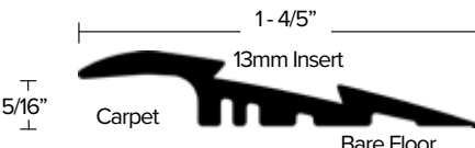
DT028 Carpet to Floor Transition SAFETY TRANSITION FOR USE FROM CARPET TILE TO NOTHING. PRE-DRILLED AND COUNTER-SUNK HOLES FOR #4 SCREW 82° INSERT WIDTH: 13MM FINISH: EA, EN, BRZ, EBLK
