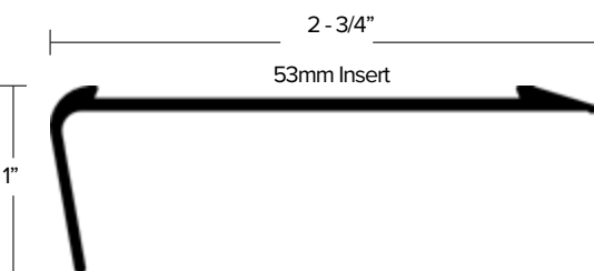
AA125 1" Rake-Back SAFETY STAIR WITH PRE-DRILLED AND COUNTER-SUNK HOLES FOR #4 SCREW 82° INSERT WIDTH: 53MM FINISH: EA, EN, BRZ
