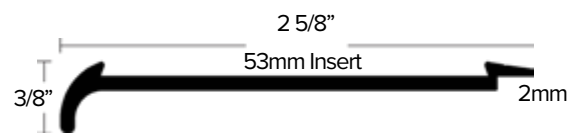
AA110 Nosing for 2mm Vinyl SAFETY STAIR WITH PRE-DRILLED AND COUNTER-SUNK HOLES FOR #4 SCREW 82° INSERT WIDTH: 53MM FINISH: EA, EN, BRZ, EBLK
