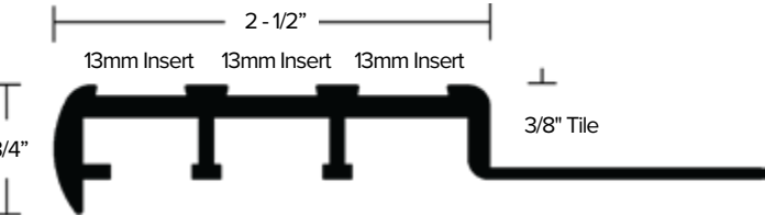
AA351 Ceramic Stair Nose SAFETY STAIR WITH PRE-DRILLED AND COUNTER-SUNK HOLES FOR #4 SCREW 82° INSERT WIDTH: 13MM X 3 FINISH: EA, EN, BRZ
