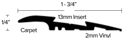
DT024 Sheet Vinyl Transition SAFETY TRANSITION FOR USE BETWEEN 2MM SHEET VINYL AND CARPET. PRE-DRILLED AND COUNTER-SUNK HOLES FOR #4 SCREW 82° INSERT WIDTH: 13MM FINISH: EA, EN, BRZ, EBLK
