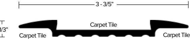
DT026 Safety Joiner SAFETY JOINER FOR USE WITH CARPET TILE. PRE-DRILLED AND COUNTER-SUNK HOLES FOR #4 SCREW 82° FINISH: EA, EN, BRZ, EBLK
