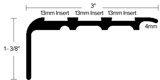
AA346 13/8" Right Angle Drop SAFETY STAIR WITH PRE-DRILLED AND COUNTER-SUNK HOLES FOR #4 SCREW 82° INSERT WIDTH: 13MM X 3 FINISH: EA, EN, BRZ
