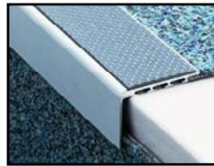
AA123 2" Right Angle Drop SAFETY STAIR WITH PRE-DRILLED AND COUNTER-SUNK HOLES FOR #4 SCREW 82° INSERT WIDTH: 53MM FINISH: EA, EN, BRZ
