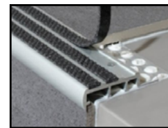
AA351 Ceramic Stair Nose SAFETY STAIR WITH PRE-DRILLED AND COUNTER-SUNK HOLES FOR #4 SCREW 82° INSERT WIDTH: 13MM X 3 FINISH: EA, EN, BRZ
