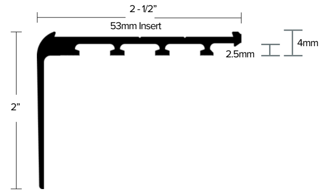
AA123 2" Right Angle Drop SAFETY STAIR WITH PRE-DRILLED AND COUNTER-SUNK HOLES FOR #4 SCREW 82° INSERT WIDTH: 53MM FINISH: EA, EN, BRZ
