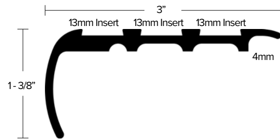
AA345 13/8" Bullnose BULLNOSE SAFETY STAIR WITH PRE-DRILLED AND COUNTER-SUNK HOLES FOR #4 SCREW 82° INSERT WIDTH: 13MM X 3 FINISH: EA
