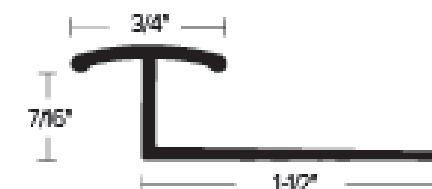
CM 212 3/4" PINLESS JOINER FINISH: HMF, HB, HEA, HN
