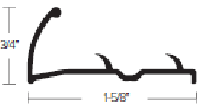
CM 99A 3/4" PREMIUM PIN CLAMPDOWN FINISH: HMF, HB, HN, HBDB, CVG, HBRZ, HMF-FLEX, HB-FLEX, HN-FLEX, HBRZ-FLEX
