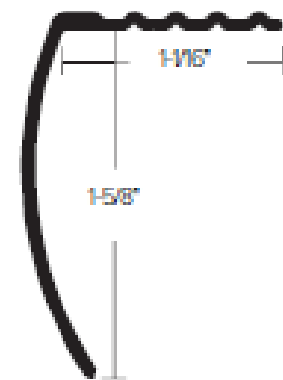
CM 605 1-5/8" DELUXE STAIR NOSING FINISH: HMF, HB, HEA, HN, HBDB, CVG, HBRZ
