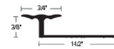
CM 208 3/4" PALISADE PINLESS JOINER FINISH: HMF, HB, HEA, HN
