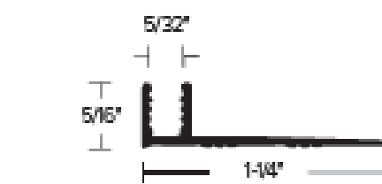
CM 210 5/16" VINYL INSERT PINLESS METAL FINISH: MF, MF-FLEX
