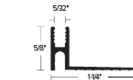
CM 215 5/8" VINYL INSERT PINLESS METAL / EXTENDER FINISH: MF
