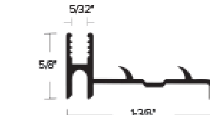
CM 115 5/8" VINYL INSERT CARPET METAL WITH PINS / EXTENDER FINISH: MF
