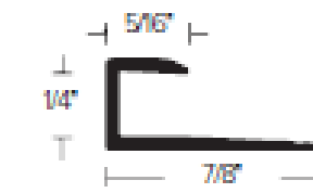
CM 401 1/4" COVING CAP FINISH: HMF, MFA, BA, HB, MFB, EN
