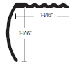
CM 601 1 - 1/16" DELUXE STAIR NOSING FINISH: HMF, HB, HN, HBDB, CVG, OAK, CHERRY, GUNSTOCK
