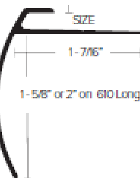
LVT 608 STAIR NOSING SIZE: 2.5mm - LVT 625 3mm - LVT 630 4mm - LVT 606 5mm - LVT 608 5mm - LVT 610 (Long) 6mm - LVT 604 7mm - LVT 612 8mm - LVT 618 FINISH: EA, EN, BRZ *7 & 8mm have "recessed lip" to cover exposed "click lock" systems.
